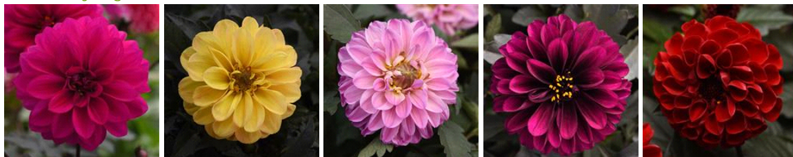
Neon
